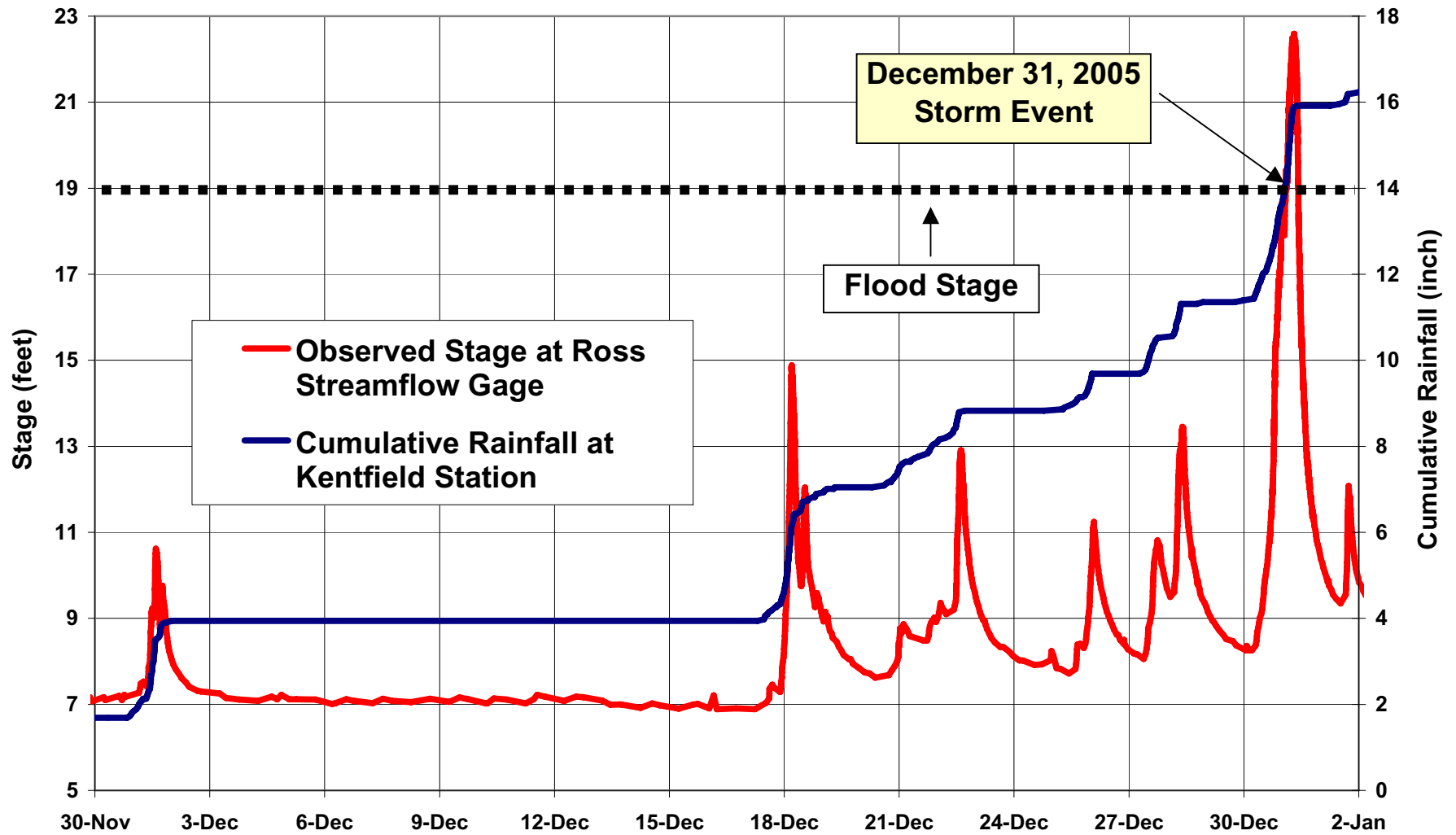
Streamflow Stage at Ross Gage, and Cumulative Rainfall at Kentfield December 2005
